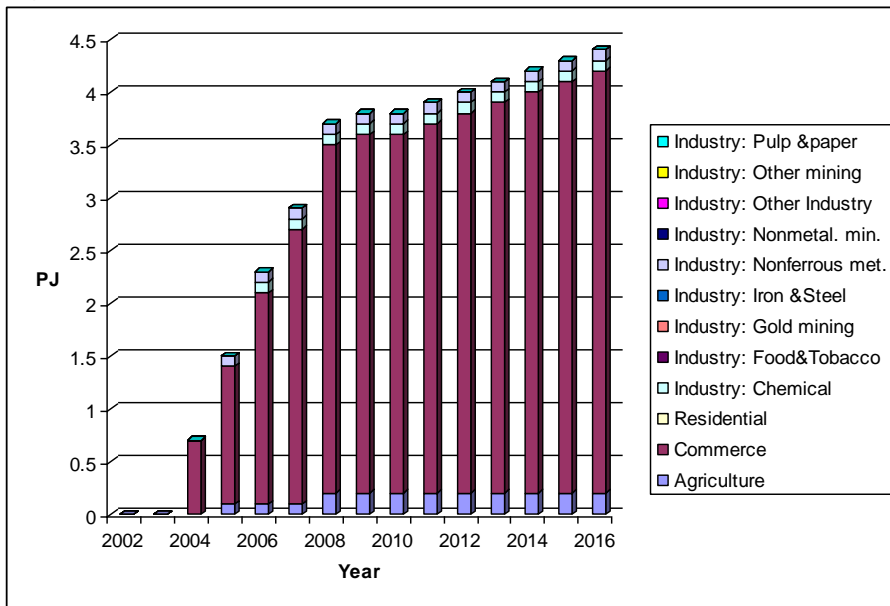
Figure 11: Efficiently operated HVAC systems
